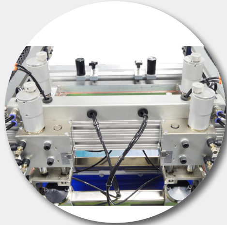
Solid chopper assembly on upgraded units provides consistent, even ink deposit and reduces deflection.
